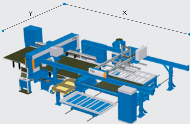
Combi Genius with LSR CG 1530: Y 9.2 m, X 14.6 m CG 1540: Y 9.2 m, X 18.5 m
