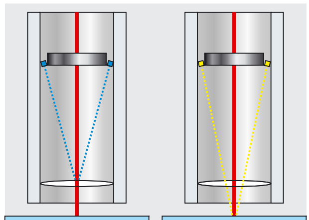
Lens condition sensor LCS
