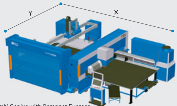
Combi Genius with Compact Express CG 1225: Y 6.2 m, X 7.8 m CG 1530: Y 6.8 m, X 9.0 m
